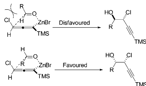
Scheme 3. Proposed Transition State Model for Selectivity
