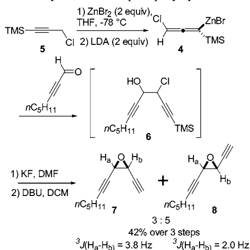
Scheme 2. Preparation of the Allenyl Zinc Bromide and the Synthesis of Simple Epoxydiynes
