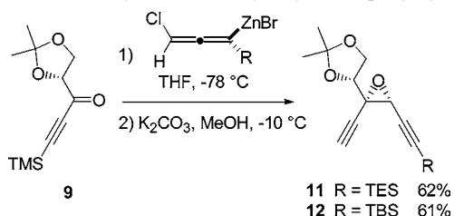
Scheme 7. Synthesis of Key Silylated Epoxydiynes
