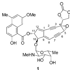
Figure 1. Neocarzinostatin chromophore.
