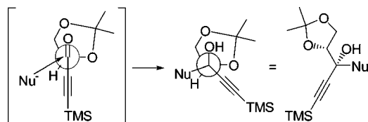
Scheme 5. Proposed Stereoselective Nucleophilic Attack on 9
