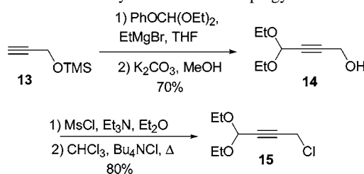
Scheme 8. Synthesis of the Propargyl Chloride
