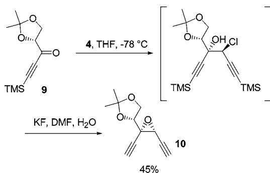
Scheme 6. Addition to a Chiral Ketone
